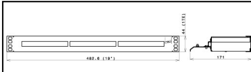
Dimension drawing of 19" enclosure
