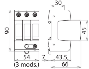
Dimension drawing DG MU 3PY 208 3W+G
