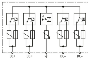
Basic circuit diagram DCU YPV SCI 1000 2M
