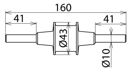
Dimension drawing TFS
