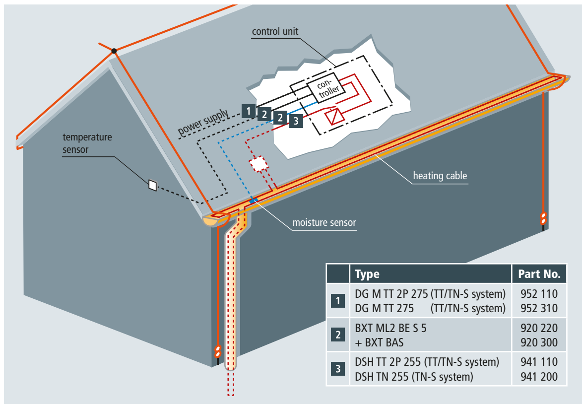
Figure 2 Installation of lightning current and surge arresters if the control unit is located far from the entry point into a structure with external lightning protection system
