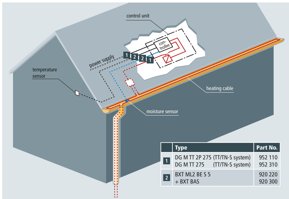
Figure 1 Control unit protected by surge arresters in a structure without external lightning protection system
