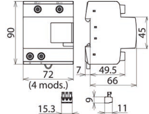
Dimension drawing DCB YPV 1200 FM
