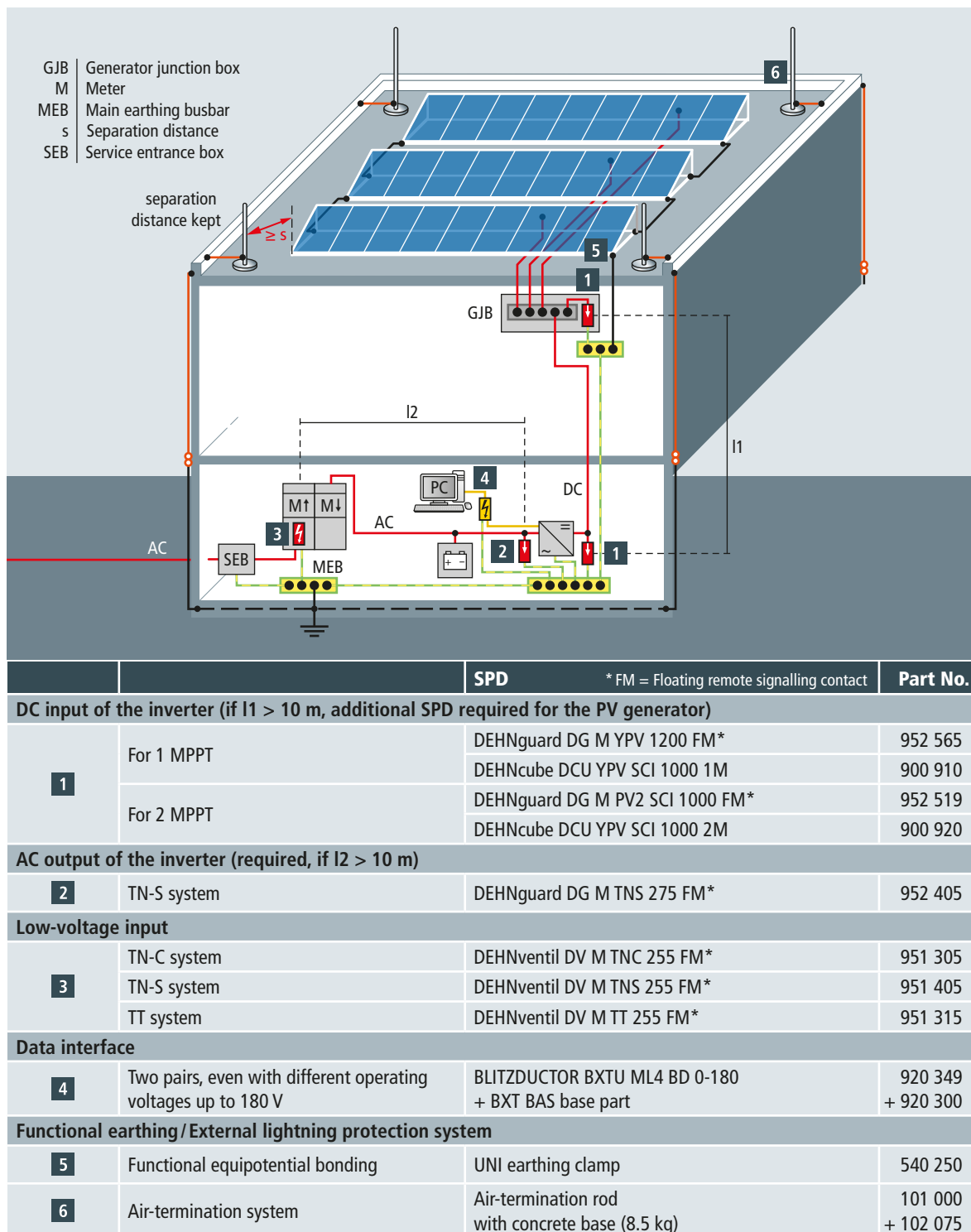
Figure 11 PV system installed on a building with external LPS and sufficient separation distance
