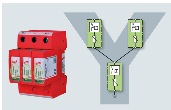
Figure 7 Modular DEHNGuard M YPV ... (FM) type 2 surge arrester with fault-resistant Y circuit
