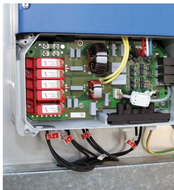
Figure 9 DEHNGuard type 2 SPD integrated in the inverter for the DC side
