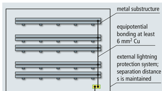
Figure 1 Functional earthing of the mounting systems if no external lightning protection system is installed or the separation distance is maintained (DIN EN 62305-3, Supplement 5)
