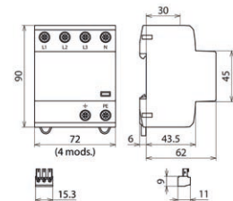
Dimension drawing DSH B TNS 255 FM
