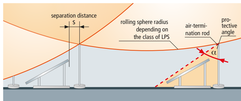
Figure 13 Rolling sphere method versus protective angle method for determining the protected volume
