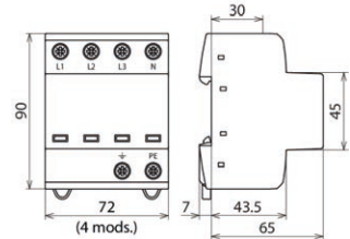
Dimension drawing DSH TNS 255
