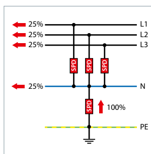
3+1 configuration with an increased discharge capacity 4 \times 20 \text{ kA} = 80 \text{ kA} .
