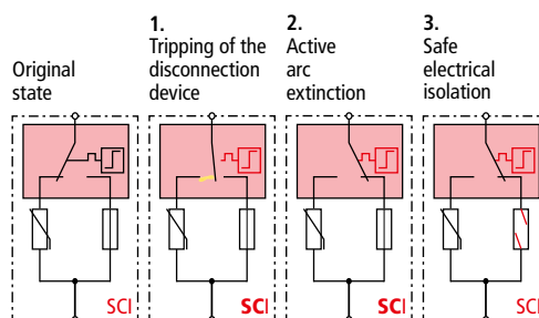
Three-step d.c. switching device (patented SCI principle)
