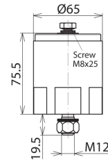
Dimension drawing V SCP 1 480
