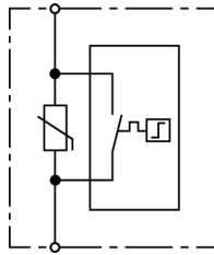
Basic circuit diagram V SCP 1 480
