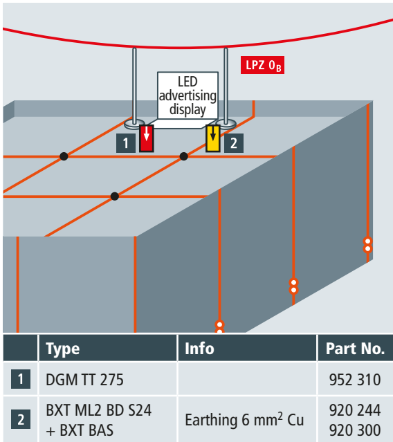
Figure 10 LED illuminated advertisement in LPZ 0 B with DALI control installed on a building with external lightning protection
