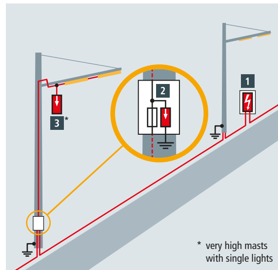
Figure 6 Lightning current flashover from the mast light housing to the mains voltage connection of the upstream device
