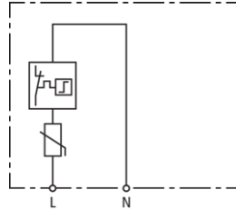
Basic circuit diagram DCOR L 1P 275
