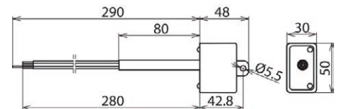
Dimension drawing DCOR L 3P 275 SO IP
