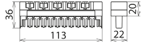
Dimension drawing DRL 10 B 180 FSD
