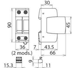
Dimension drawing DG M TN CI 275
