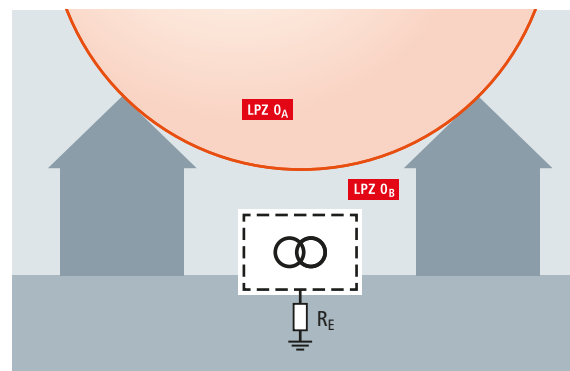
Figure 2b Rolling sphere method used for an enclosed transformer substation
