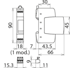
Dimension drawing DR M 2P 255 FM
