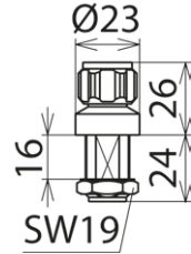
Dimension drawing DGA G N
