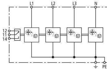
Basic circuit diagram DSH B TNS 255 FM
